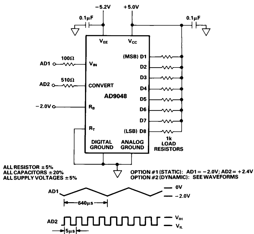
Burn-In Diagram
