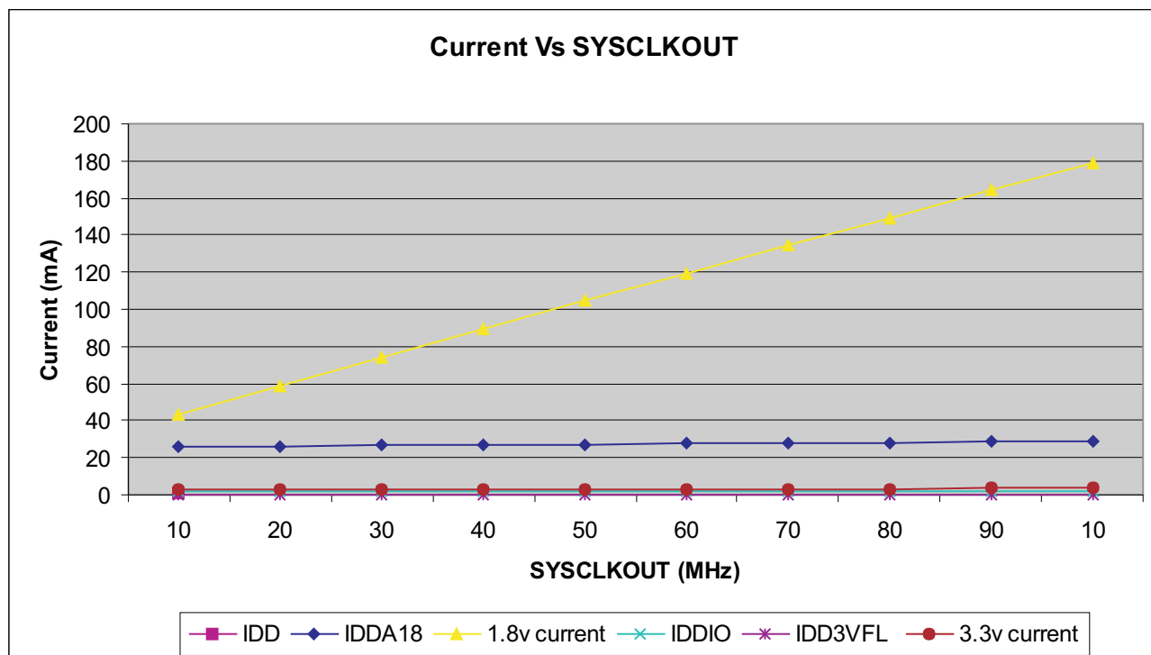
Figure 6-3. Typical Operational Current Versus Frequency (C280x)
