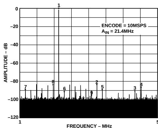
Figure 59. IF Sampling a 21.4 MHz Input Using the AD9220 ( V_{CM} = 2.5 V, Input Span = 2 V p-p)
