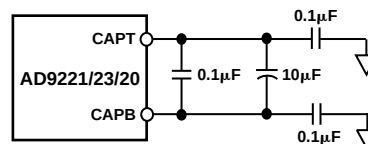
Figure 36. Recommended CAPT/CAPB Decoupling Network
