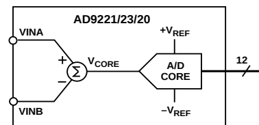
Figure 31. AD9221/AD9223/AD9220 Equivalent Functional Input Circuit
