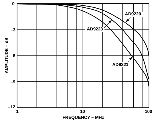
Figure 29. Full-Power Bandwidth
