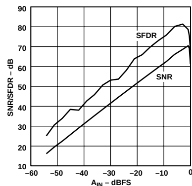
Figure 28. SNR/SFDR vs. A_{IN} (Input Amplitude) ( f_{IN} = 5.0\text{ MHz} , Input Span = 2 V p-p, V_{CM} = 2.5\text{ V} )
