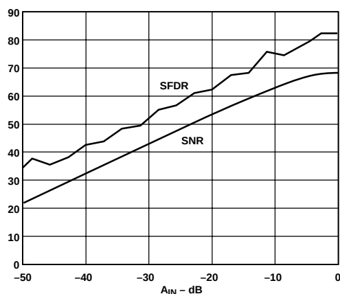
Figure 60. AD9220 Differential Input SNR/SFDR vs. Input Amplitude ( A_{IN} ) @ 21.4 MHz
