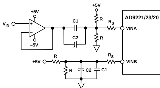
Figure 42. AC-Coupled Input-Flexible Input Span, V_{CM} = 2\text{ V}
