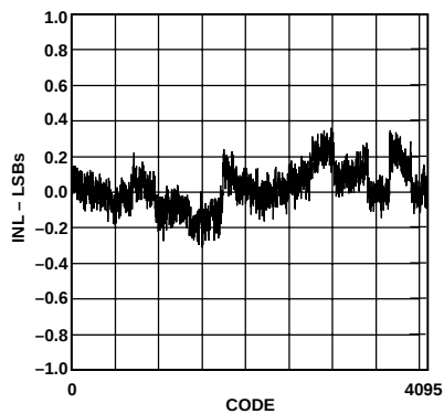
Figure 3. Typical INL
