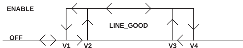
Figure 2. Line UVLO and OVLO Operation
