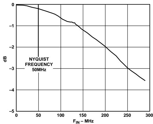
Figure 16. Frequency Response
