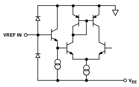
Figure 3. Equivalent Reference Input Circuit
