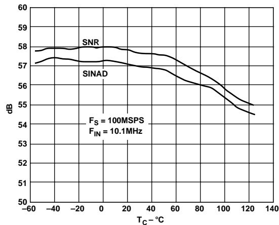
Figure 14. SNR vs. T_C : TD Package (DIP)
