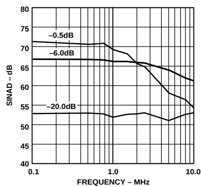
Figure 25. SINAD vs. Input Frequency (Input Span = 5.0 V p-p, V_{CM} = 2.5\text{ V} )
