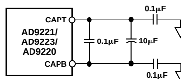
Figure 36. Recommended CAPT/CAPB Decoupling Network
