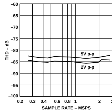
Figure 9. THD vs. Sample Rate ( A_{IN} = -0.5 \text{ dB} , f_{IN} = 500 \text{ kHz} , V_{CM} = 2.5 \text{ V} )
