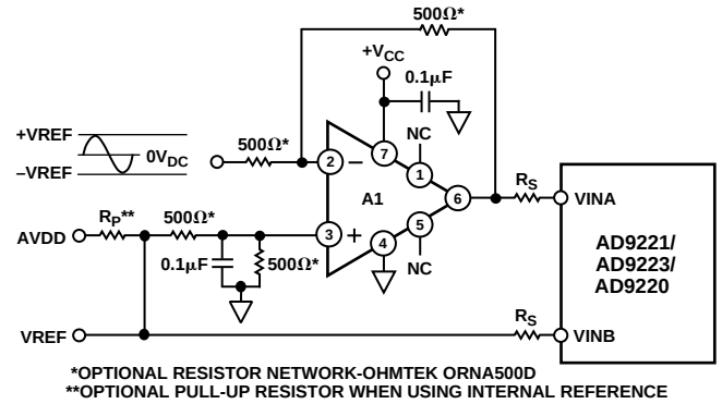
Figure 40. Single-Ended Input With DC-Coupled Level Shift
