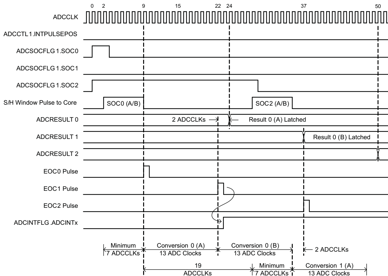
Figure 6-25. Timing Example For Simultaneous Mode/Early Interrupt Pulse
