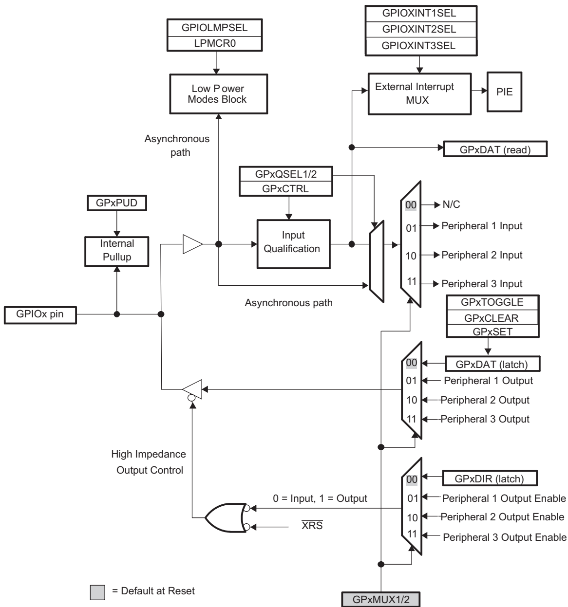
Figure 4-12. GPIO Multiplexing
