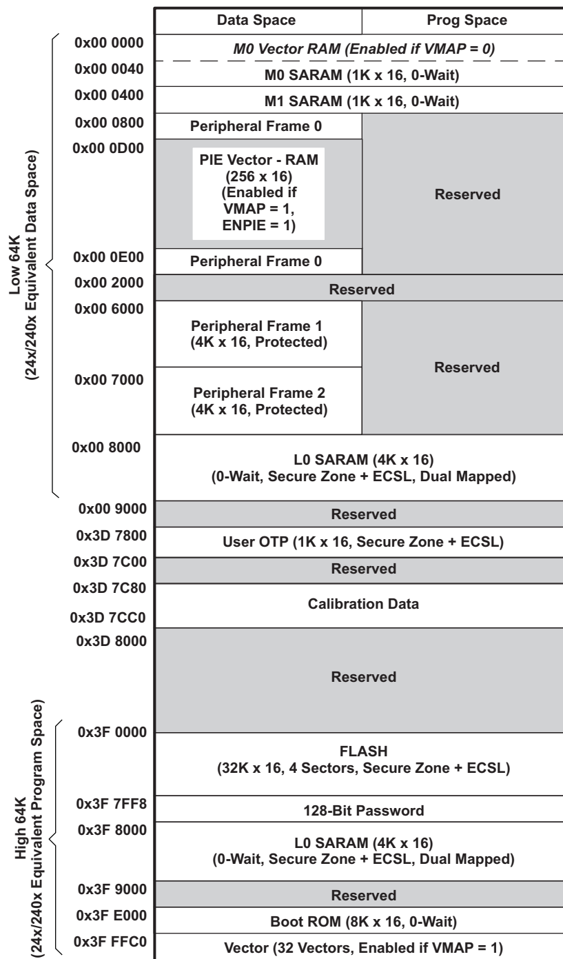
Figure 3-5. 28023/28027 Memory Map
