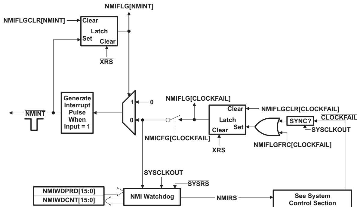
Figure 3-13. NMI-watchdog
