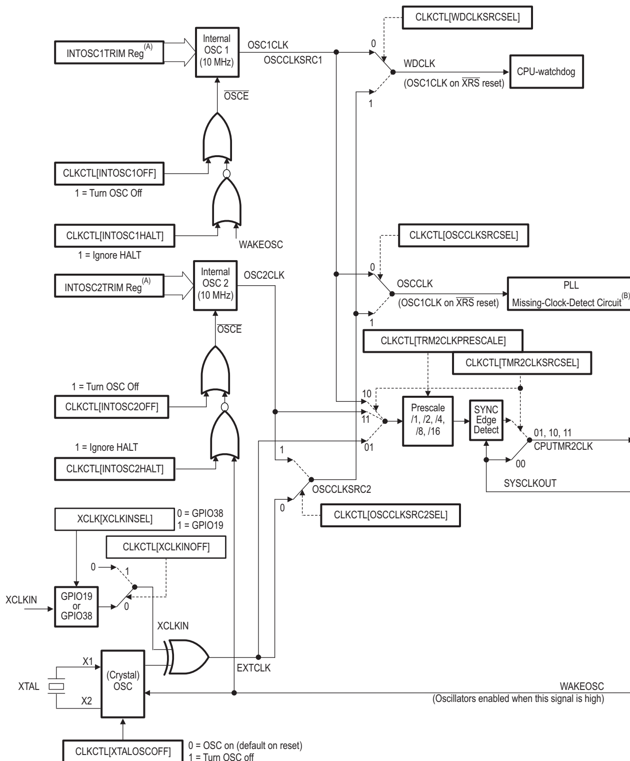
Figure 3-10. Clock Tree
