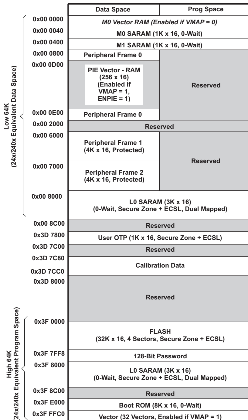
Figure 3-3. 28021 Memory Map
