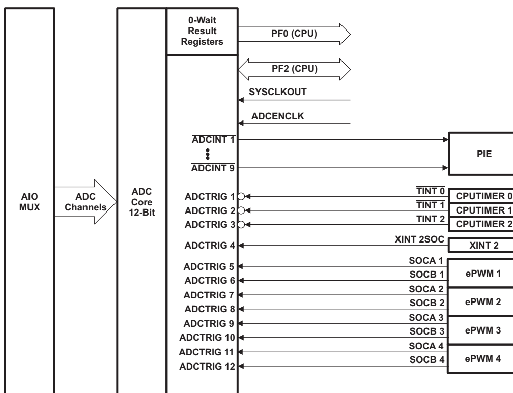
Figure 4-2. ADC Connections
