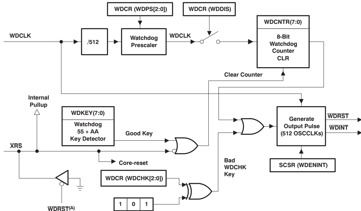
Figure 3-14. CPU-watchdog Module
