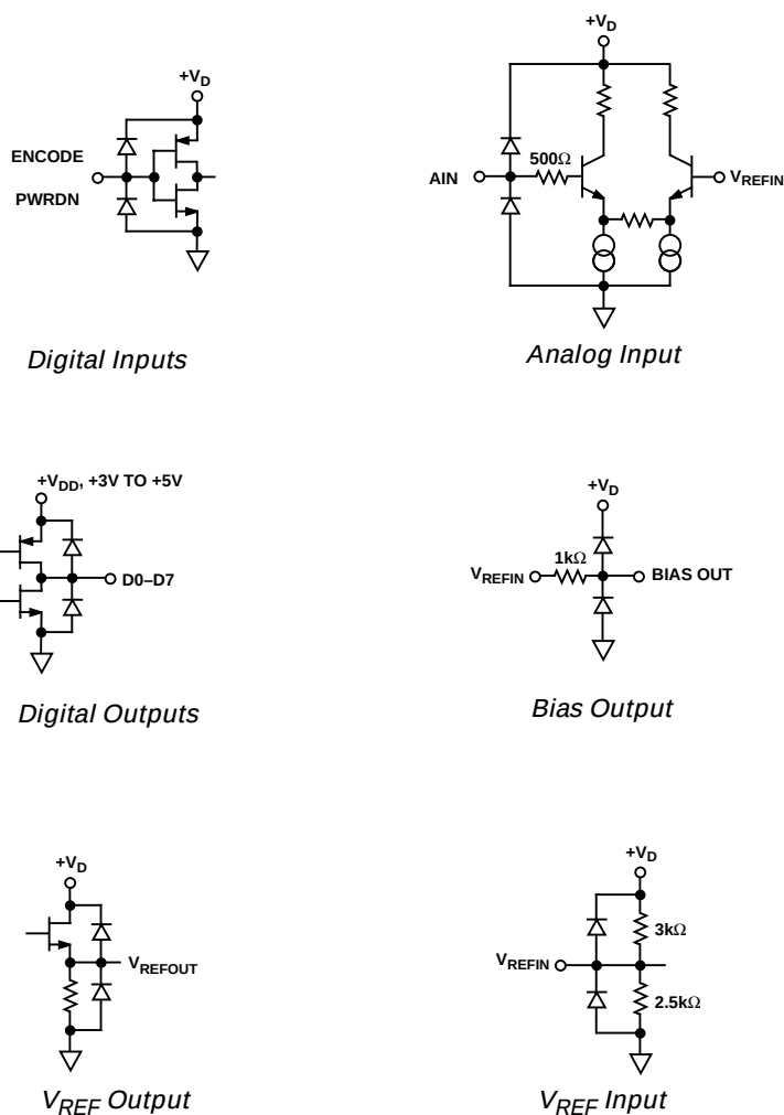
Figure 18. Equivalent Circuits
