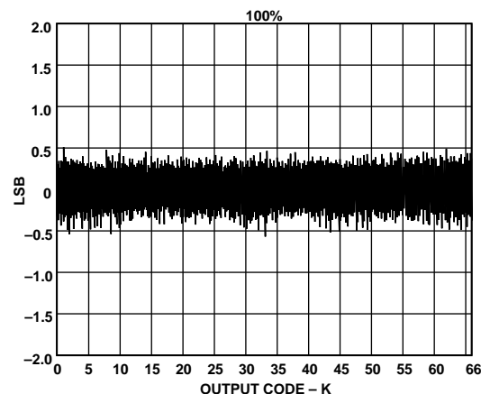
Figure 19. DNL Plot
