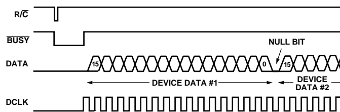
Figure 26. TAG Timing Diagram for Two Concatenated AD977/AD977As
