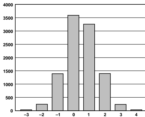
Figure 24. Histogram of 10,000 Conversions of a DC Input
