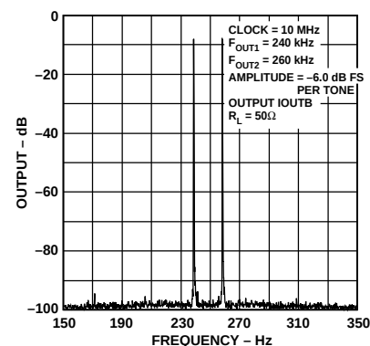
Figure 20. Intermodulation Distortion
