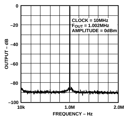
Figure 17. Typical SFDR (With a Window)
