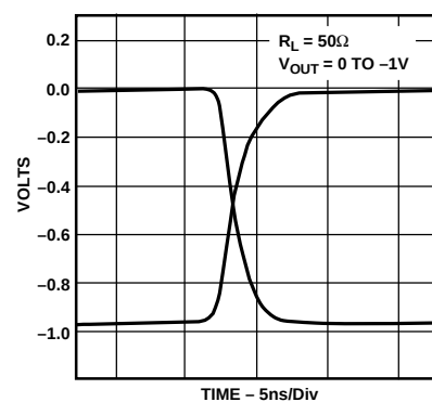
Figure 14. Rise and Fall Characteristics
