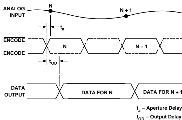
AD9060 Timing Diagram
