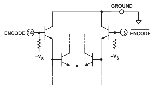
AD9060 Encode and \overline{\text{Encode}} Equivalent Circuits
