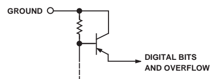
AD9060 Equivalent Digital Outputs
