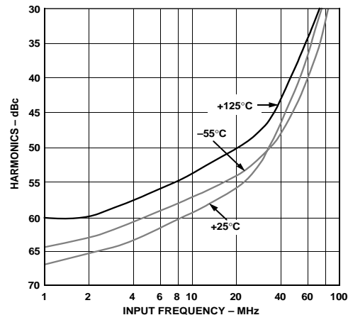
AD9060 Harmonics vs. Input Frequency
