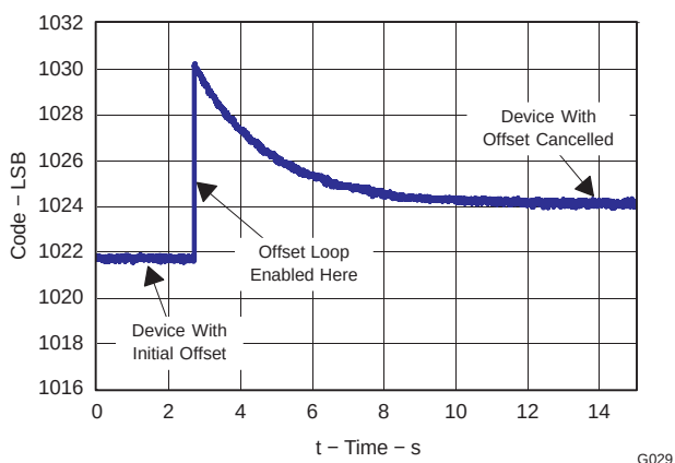
Figure 50. Time Response of Offset Correction
